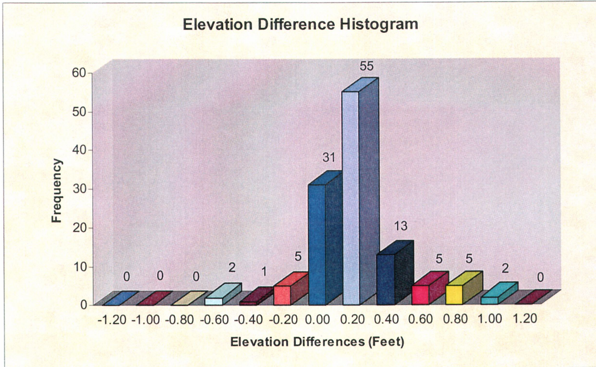
Figure 4 – Histogram of Elevation Discrepancies within 0.2 ft bands
