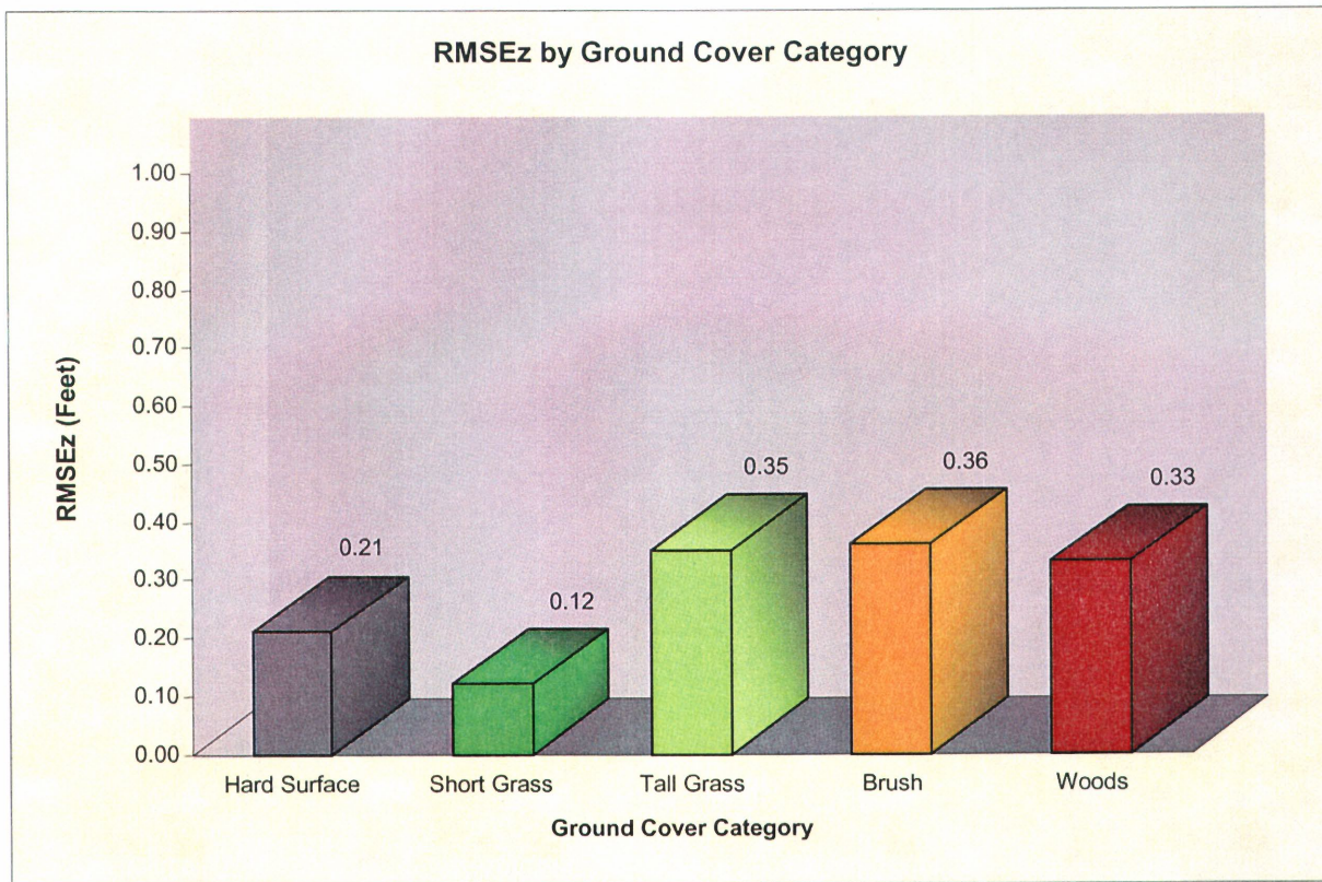
Figure 3 – RMSE_z statistics by Ground Cover Category
