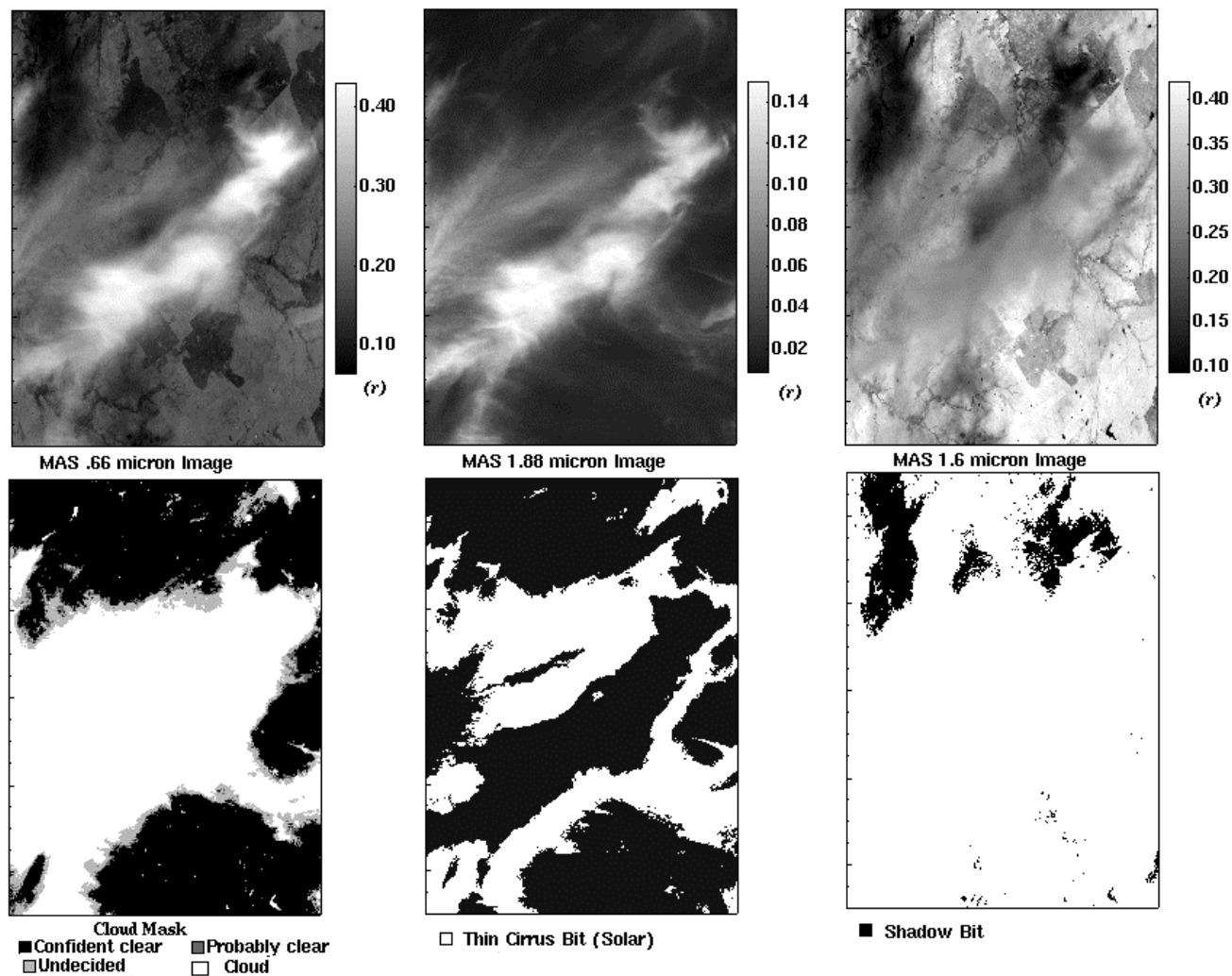
Figure 6. Example of cloud mask algorithms applied to MAS data on 26 April 1996. The upper panels are MAS images at 0.66, 1.88, and 1.6 \mu\text{m} . The lower images show the final mask, thin cirrus mask, and the shadow mask.
