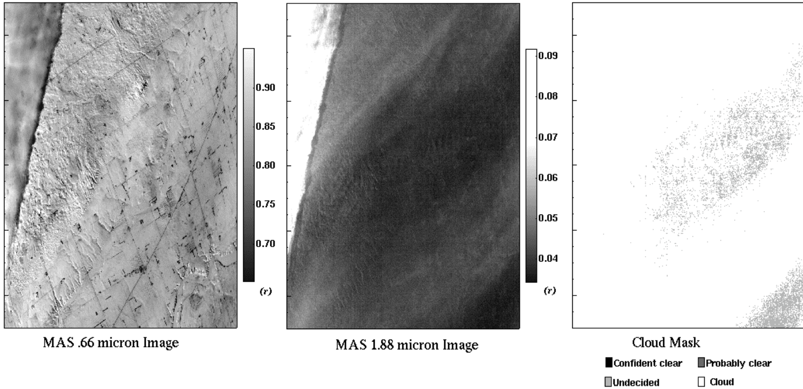
Figure 7. Example of the cloud mask algorithm applied to a winter scene on 2 February 1997.
