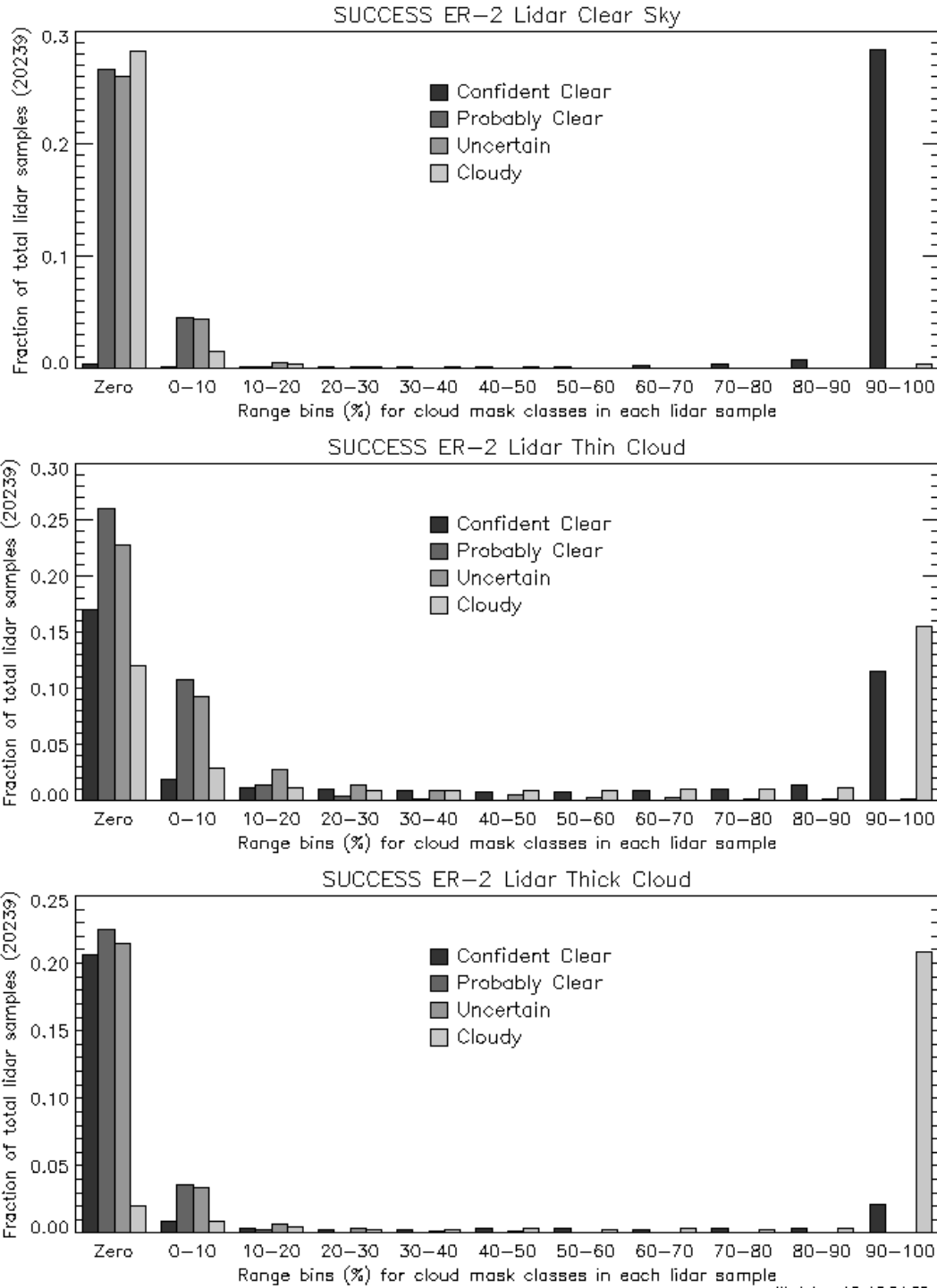
Figure 9. Comparisons between the cloud detection results using MAS and cloud lidar system for five days of the SUCCESS experiment. Cloud mask confidence is compared with three lidar categories: no cloud (top panel), thin cloud (middle panel), and thick cloud (bottom panel).
