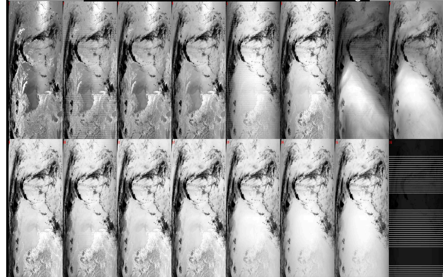
a1.16208.1740.1000m.hdf after destriping
