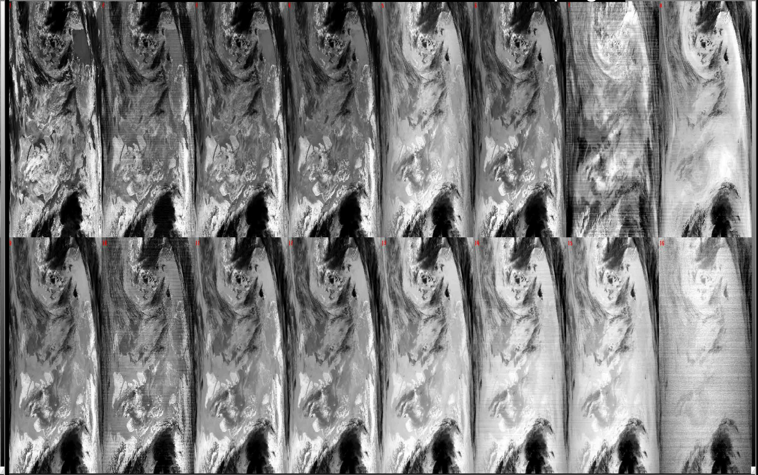
t1.16208.1910.1000m.hdf after destriping
