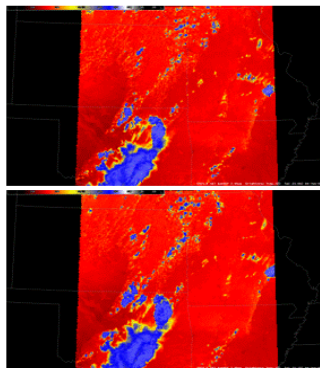
Figure 25. An example of how the ABI will scan the CONUS region routinely within an hour (i.e., 1 image every 5 minutes).
