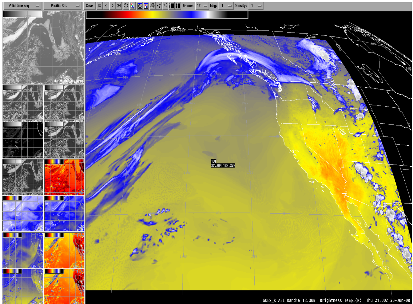
Figure 31. Shows band16 (13.3 μm) for the pacific projection on 26th-June-2008 at 21:00Z.
