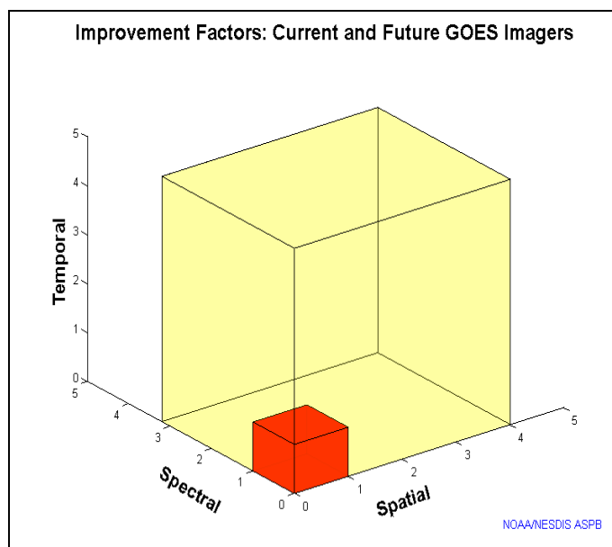
Figure 1. The comparison of the information volume between current GOES Imager (red) and the GOES-R ABI (yellow) for the spectral, spatial and temporal resolutions.
