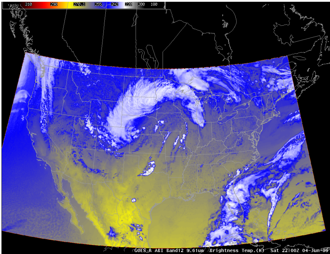
Figure 17. Simulated ABI band 12 (9.6 \mu\text{m} ) for 04 June 2005 at 22:00 UTC.
