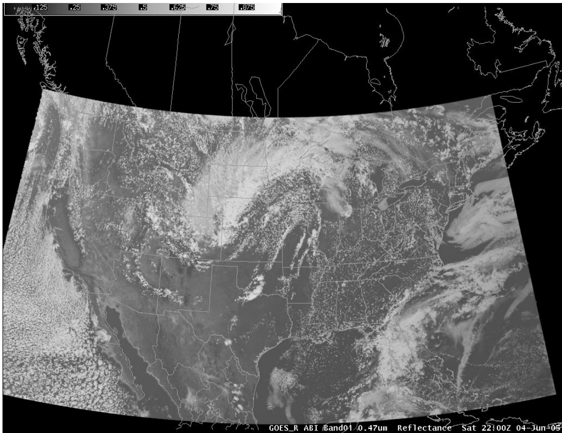
Figure 6. Simulated ABI band 1 (0.47 \mu\text{m} ) for 04 June 2005 at 22:00 UTC.
