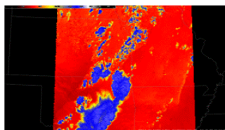
Figure 26. An example of how the current GOES imager routinely scans the CONUS region every 15 minutes, except when a full disk is being scanned there is a 30 minute gap.
