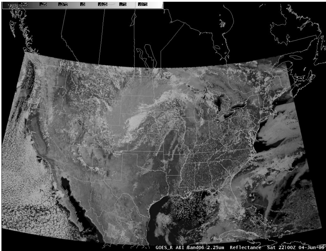
Figure 11. Simulated ABI band 6 (2.25 \mu\text{m} ) for 04 June 2005 at 22:00 UTC.
