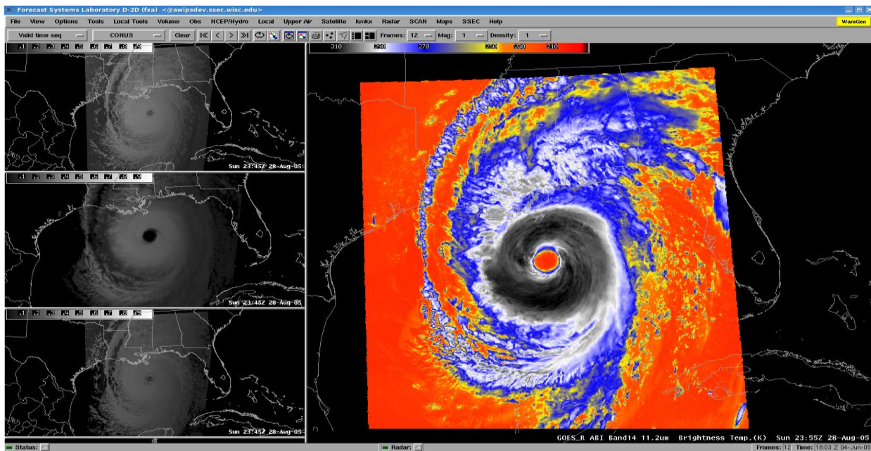
Figure 30. Four bands of the ABI are shown here from a simulated Katrina data set.
