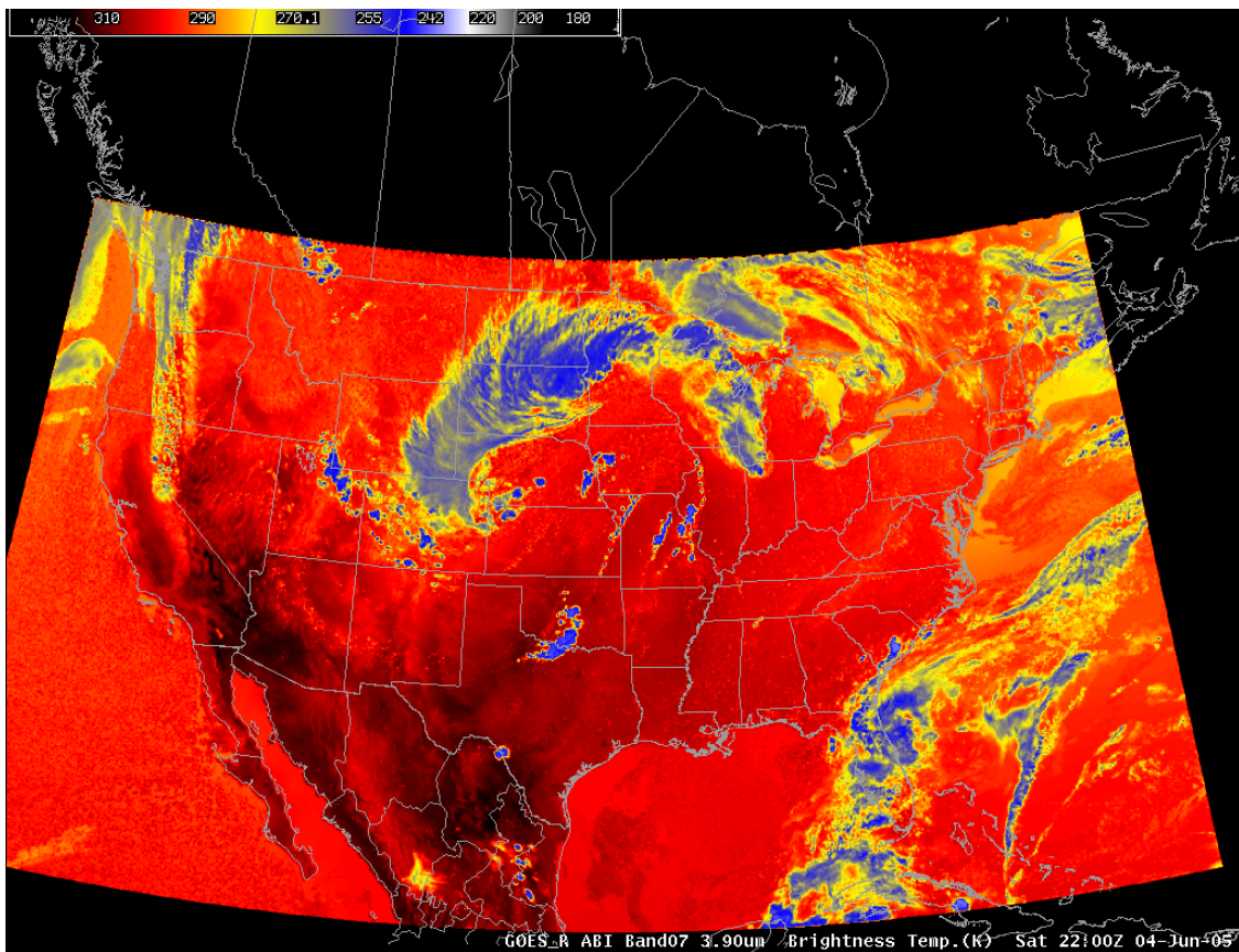
Figure 12. Simulated ABI band 7 (3.9 \mu\text{m} ) for 04 June 2005 at 22:00 UTC.
