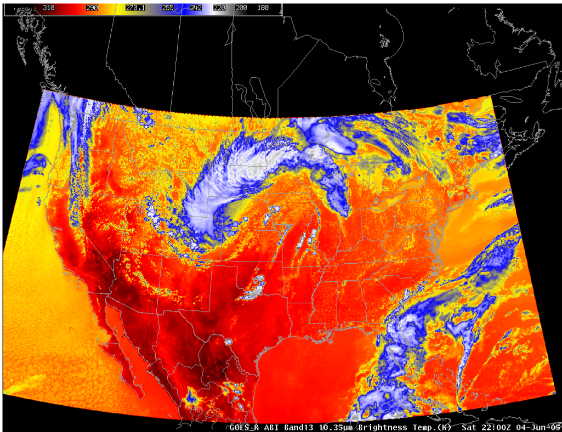
Figure 18. Simulated ABI band 13 (10.35 \mu\text{m} ) for 04 June 2005 at 22:00 UTC.
