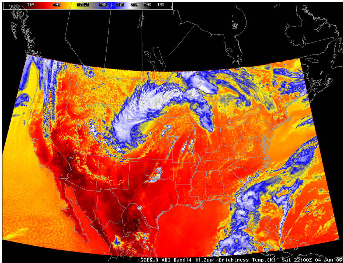
Figure 19. Simulated ABI band 14 (11.2 \mu\text{m} ) for 04 June 2005 at 22:00 UTC.
