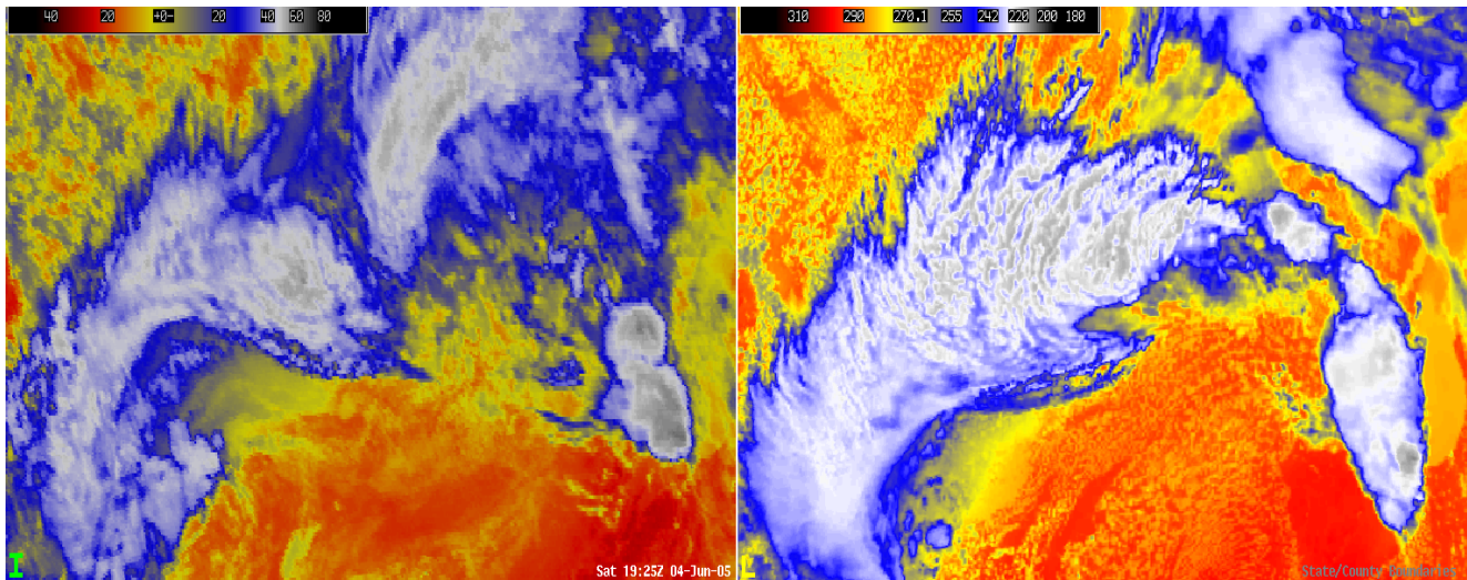
Figure 24. Example of the current GOES spatial resolution (left panel) and that expected from the ABI (right panel). The band shown here is the infrared window.
