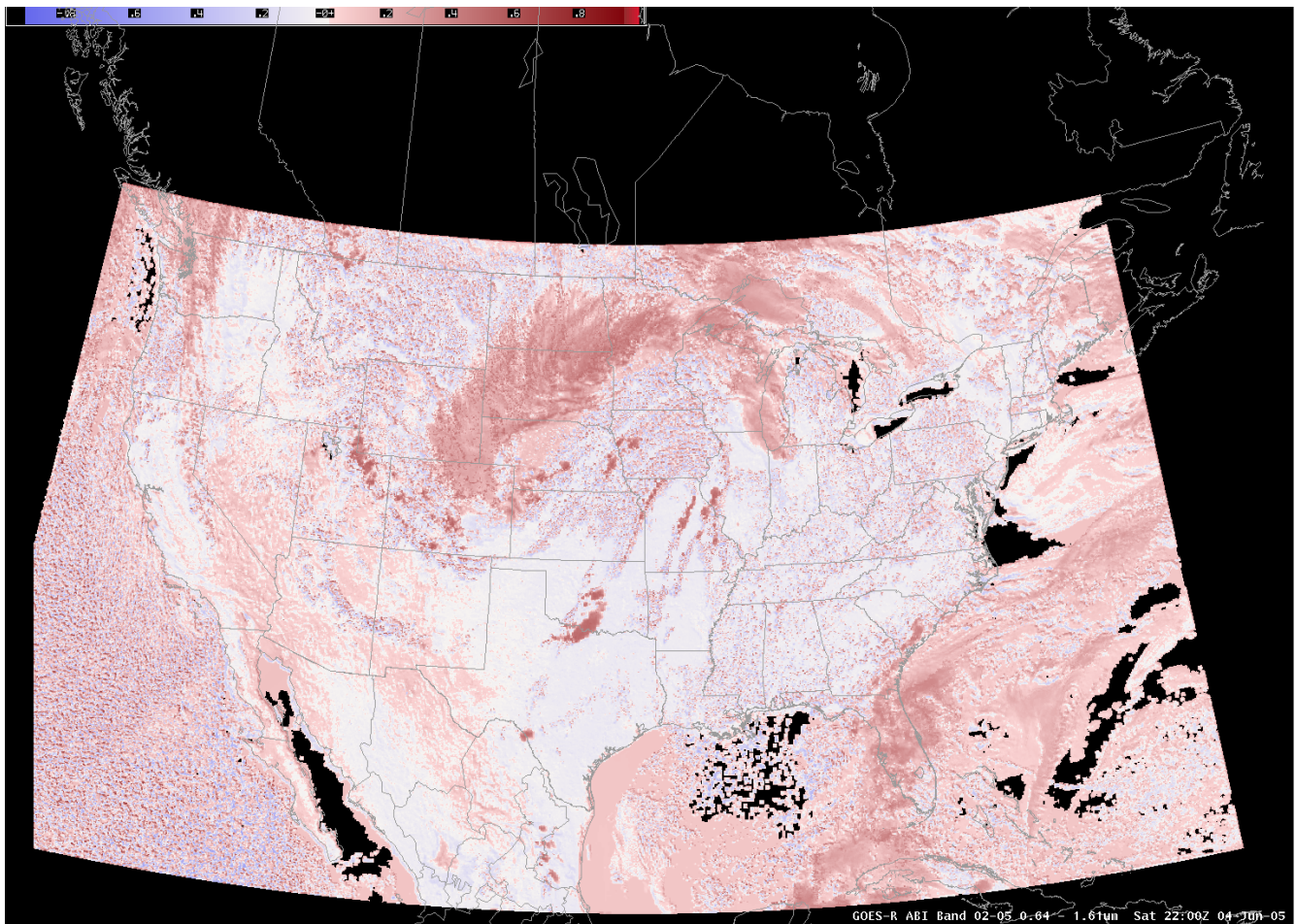
Figure 27. Example of daytime cloud phase; visible versus near-IR: Simulated ABI band 2 - 5 (e.g., 0.6 - 1.6 \mu\text{m} ). Note the different brightness temperatures differences between water and ice clouds.
