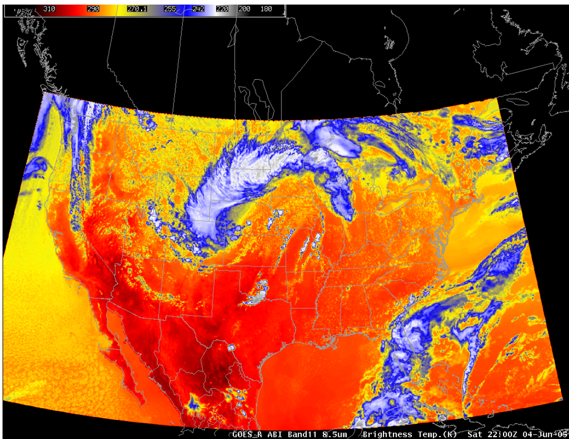
Figure 16. Simulated ABI band 11 (8.5 \mu\text{m} ) for 04 June 2005 at 22:00 UTC.
