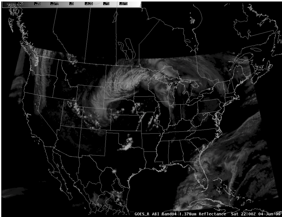
Figure 9. Simulated ABI band 4 ( 1.378 \mu\text{m} ) for 04 June 2005 at 22:00 UTC.
