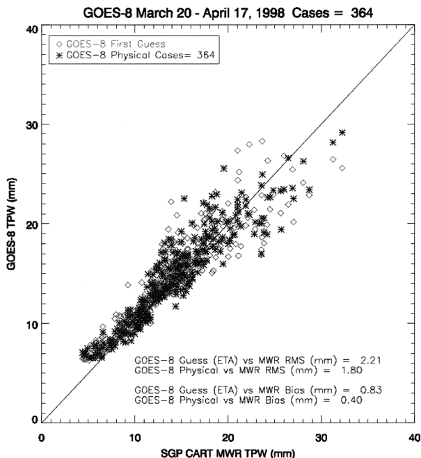
FIG. 7. A scatterplot comparing MWR total water vapor values to the Eta Model forecast (diamonds) and the GOES-8 physical retrieval (stars) values. Rms and bias for all matches are quantified in the lower-right-hand corner.
