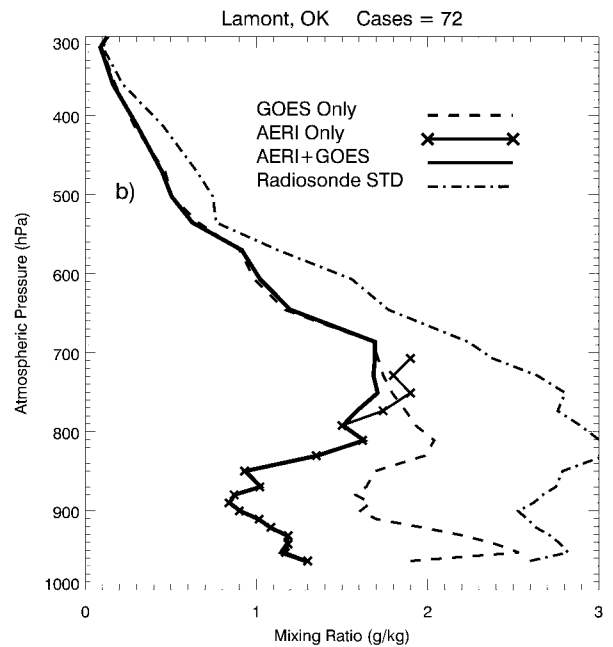
FIG. 10. (a), (b) Rms differences from 72 radiosondes for AERI retrievals (×), GOES retrievals (dashed), and AERI plus GOES retrievals (solid black) for temperature and mixing ratio, respectively, during the 1997 WVIOP. A measure of the meteorological variability of the temperature and water vapor is indicated by the dot–dash lines.
