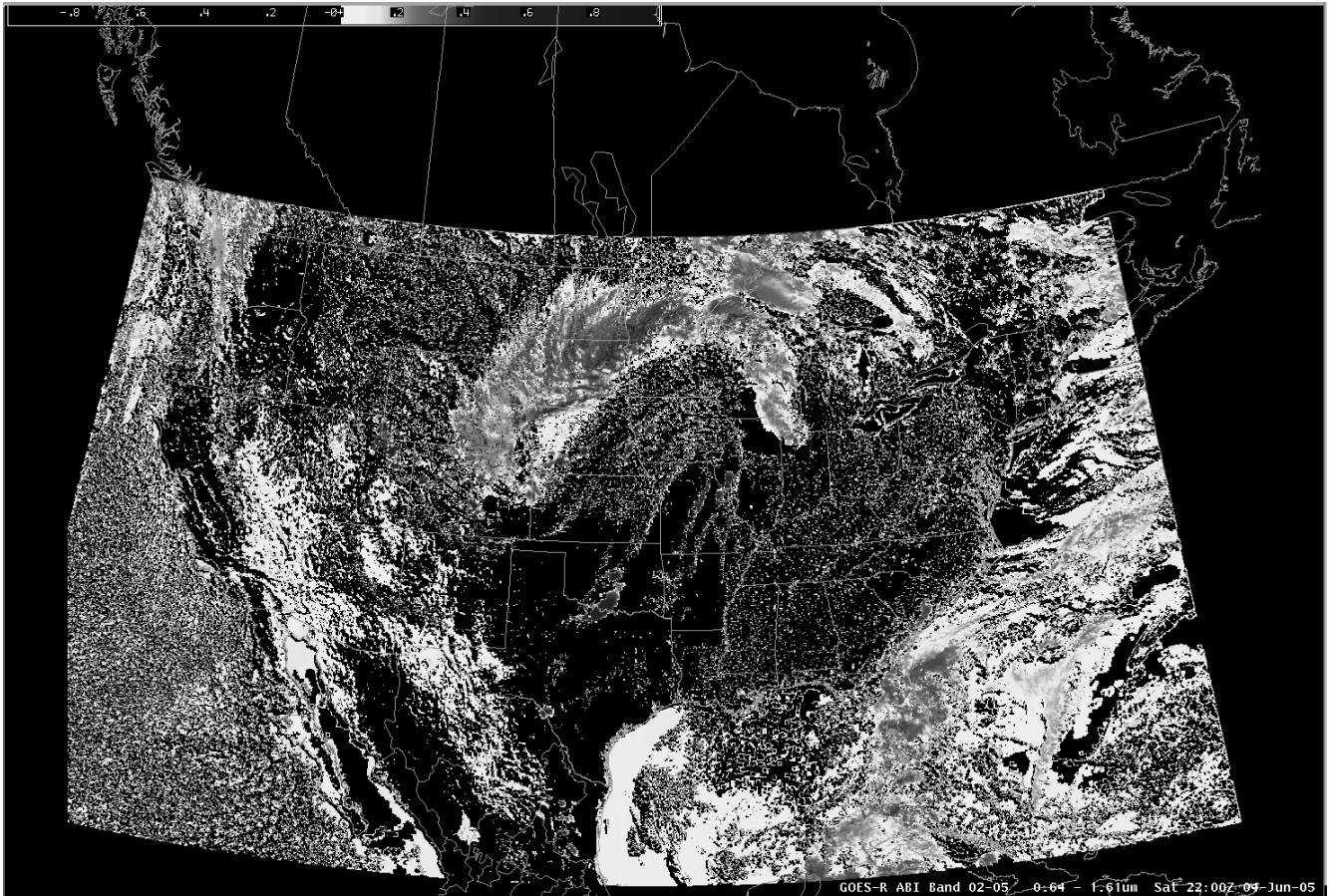
Figure 27. Example of daytime cloud phase; visible vs near-IR: Simulated ABI band 2 - 5 (eg, 0.6 - 1.6 um). Note the different brightness temperatures differences between water and ice clouds (Focused range).
