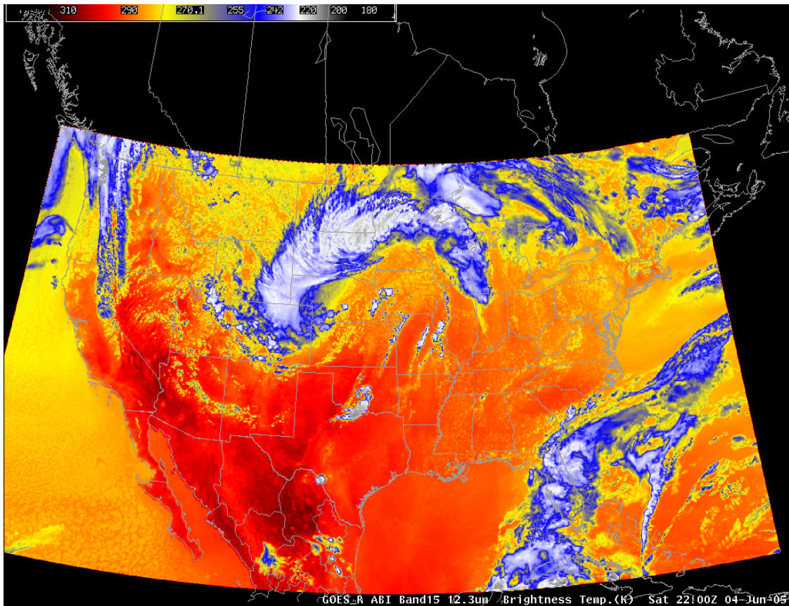
Figure 20. Simulated ABI band 15 (12.30 \mu\text{m} ) for 04 June 2005 at 22:00 UTC.
