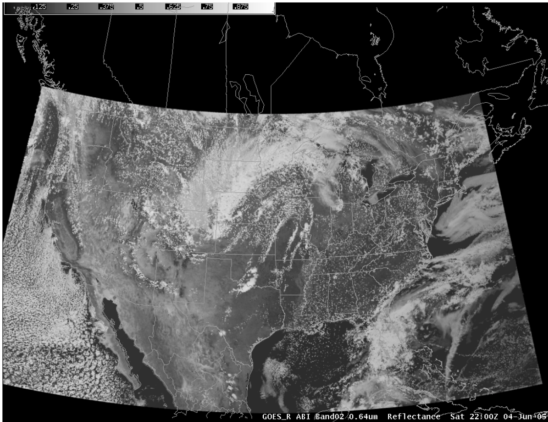
Figure 7 Simulated ABI band 02 (0.64 \mu\text{m} ) for 04 June 2005 at 22:00 UTC.
