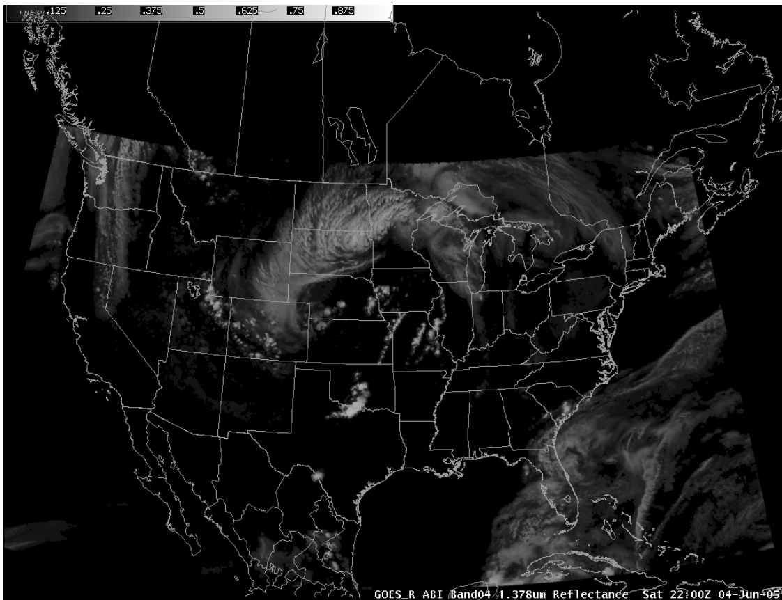
Figure 9. Simulated ABI band 04 ( 1.378\ \mu\text{m} ) for 04 June 2005 at 22:00 UTC.
