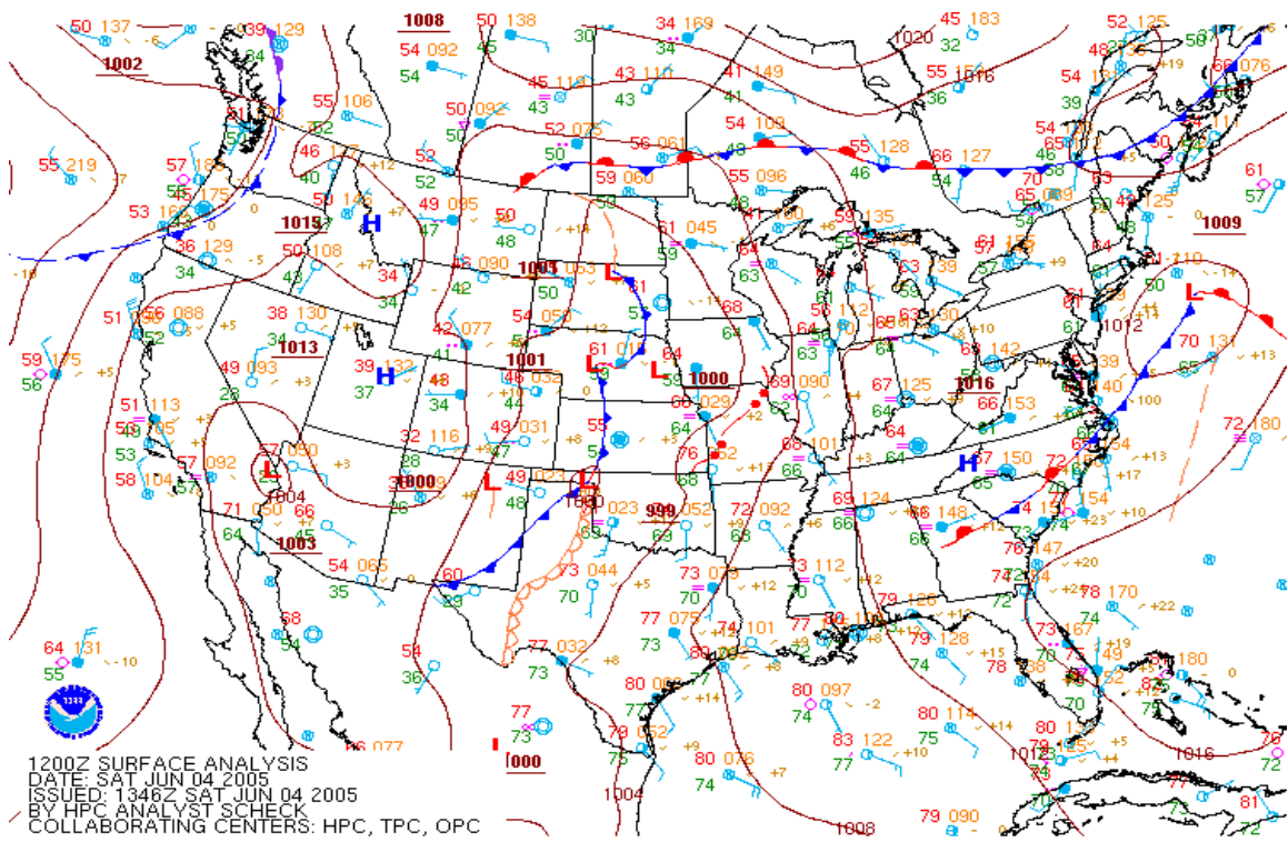
Figure 4. Surface Analysis at 12 UTC 4 June 2005. Source: Hydro meteorological Prediction Center
