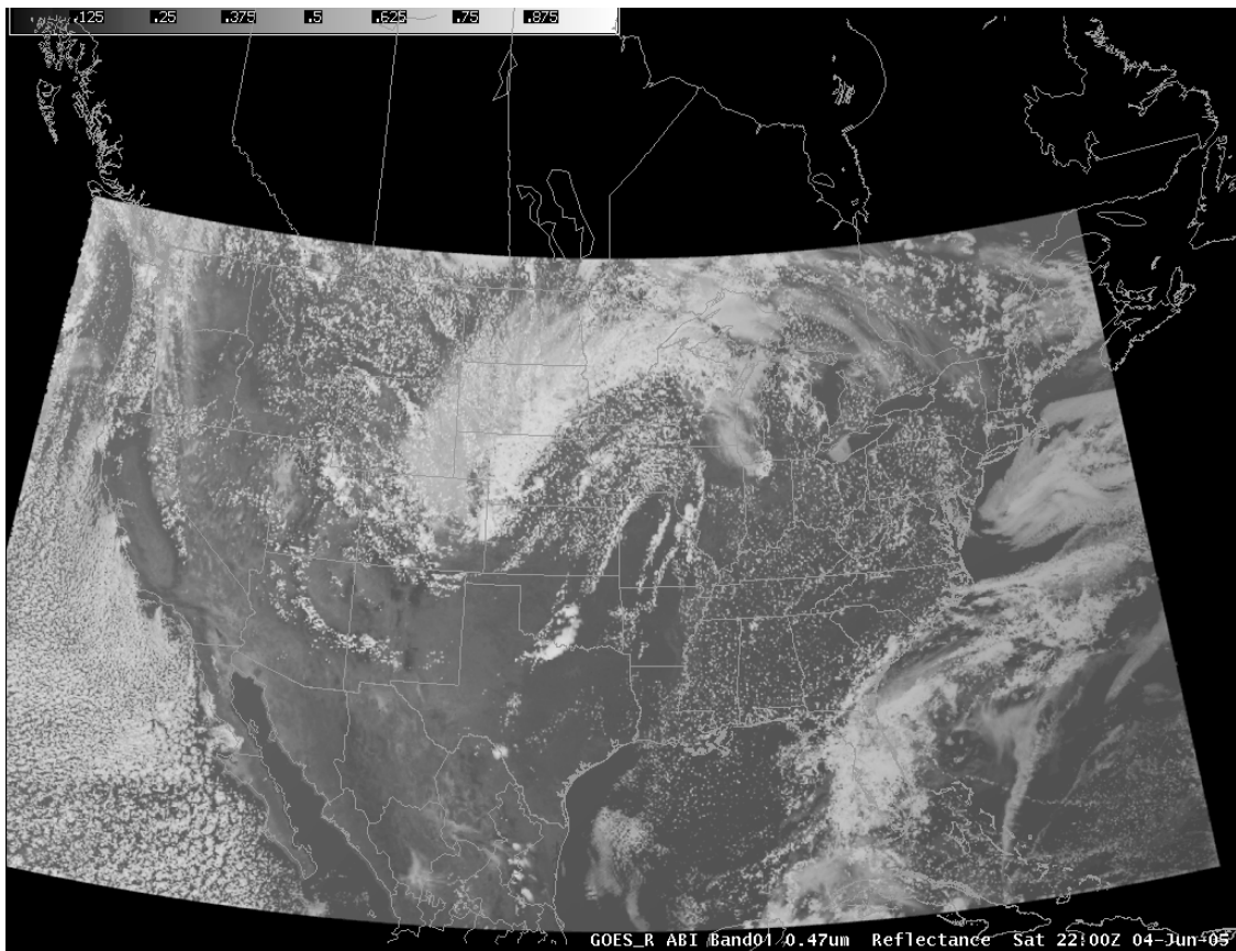
Figure 6. Simulated ABI band 01 (0.47 \mu\text{m} ) for 04 June 2005 at 22:00 UTC.
