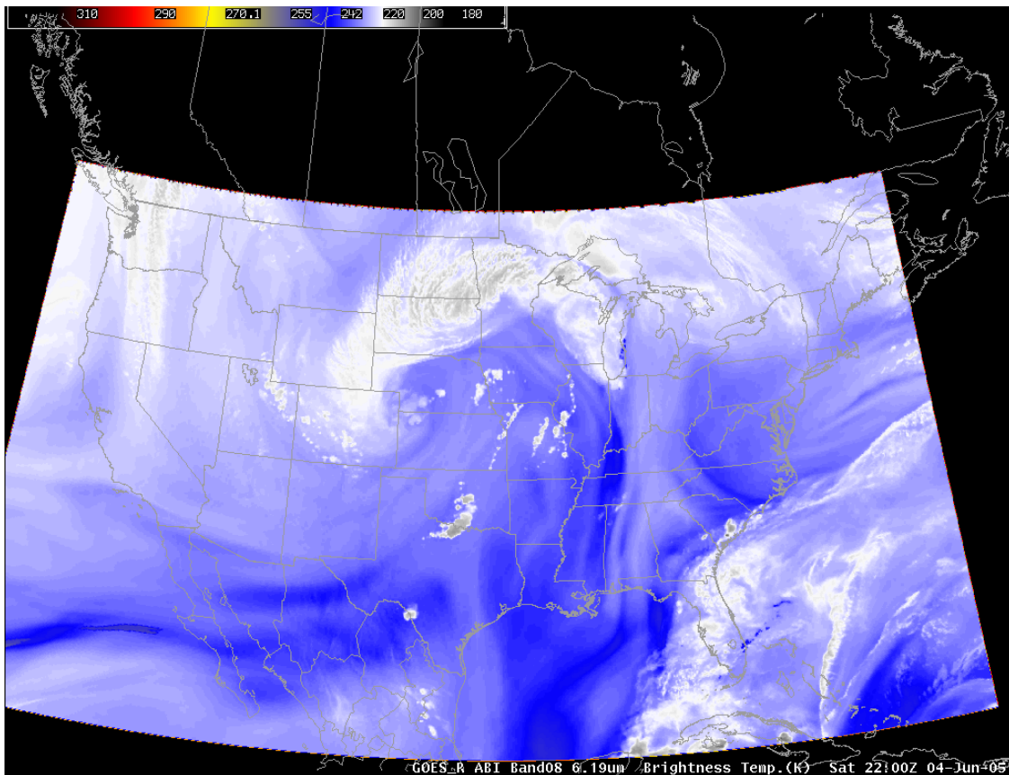
Figure 13. Simulated ABI band 08 (6.19 \mu\text{m} ) for 04 June 2005 at 22:00 UTC.
