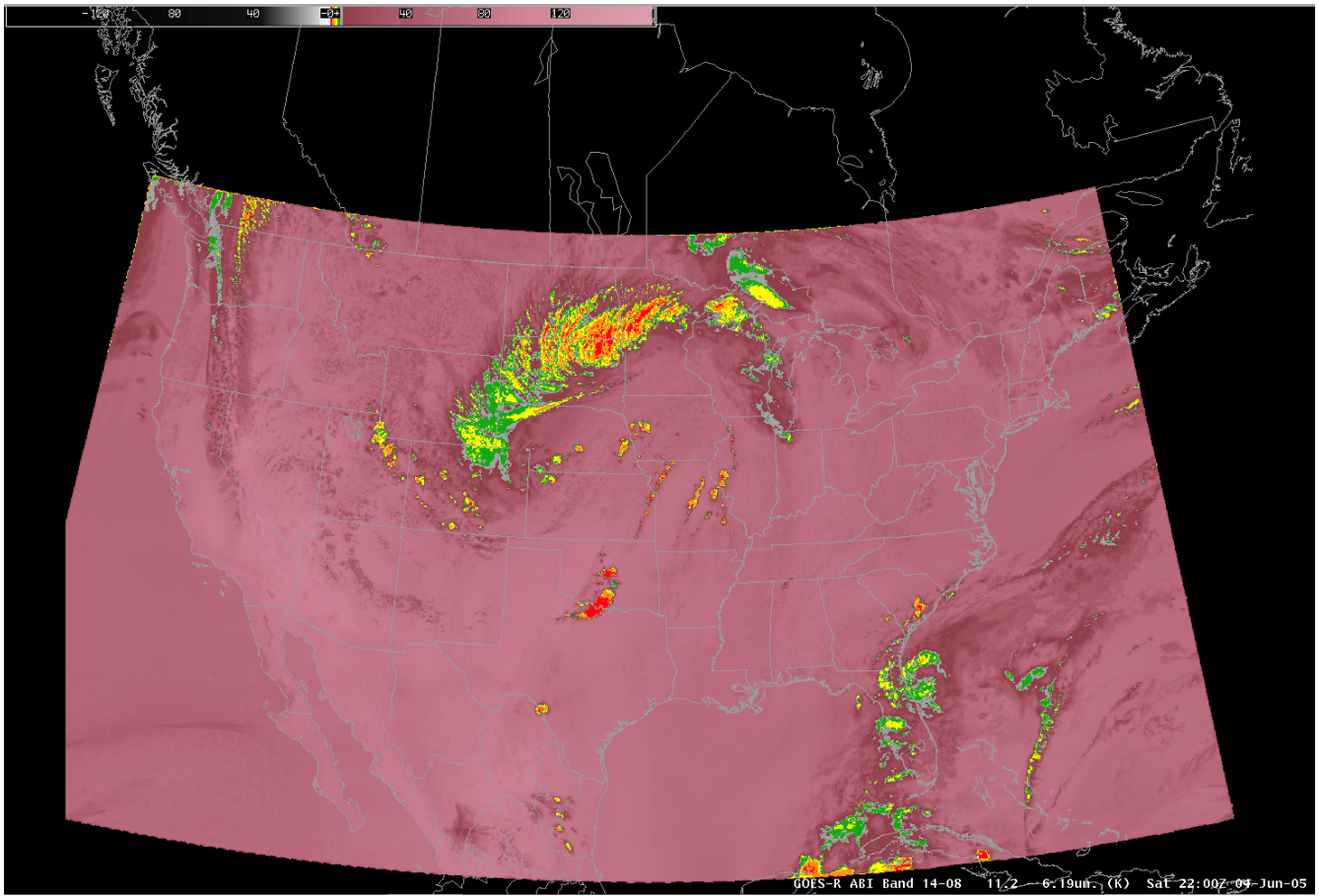
Figure 29. Upper-level information; Simulated ABI Band 14 – 08 (11.2 – 6.19 \mu m). Note the location of potentially over-shooting tops highlighted by the smallest differences (Focused range).
