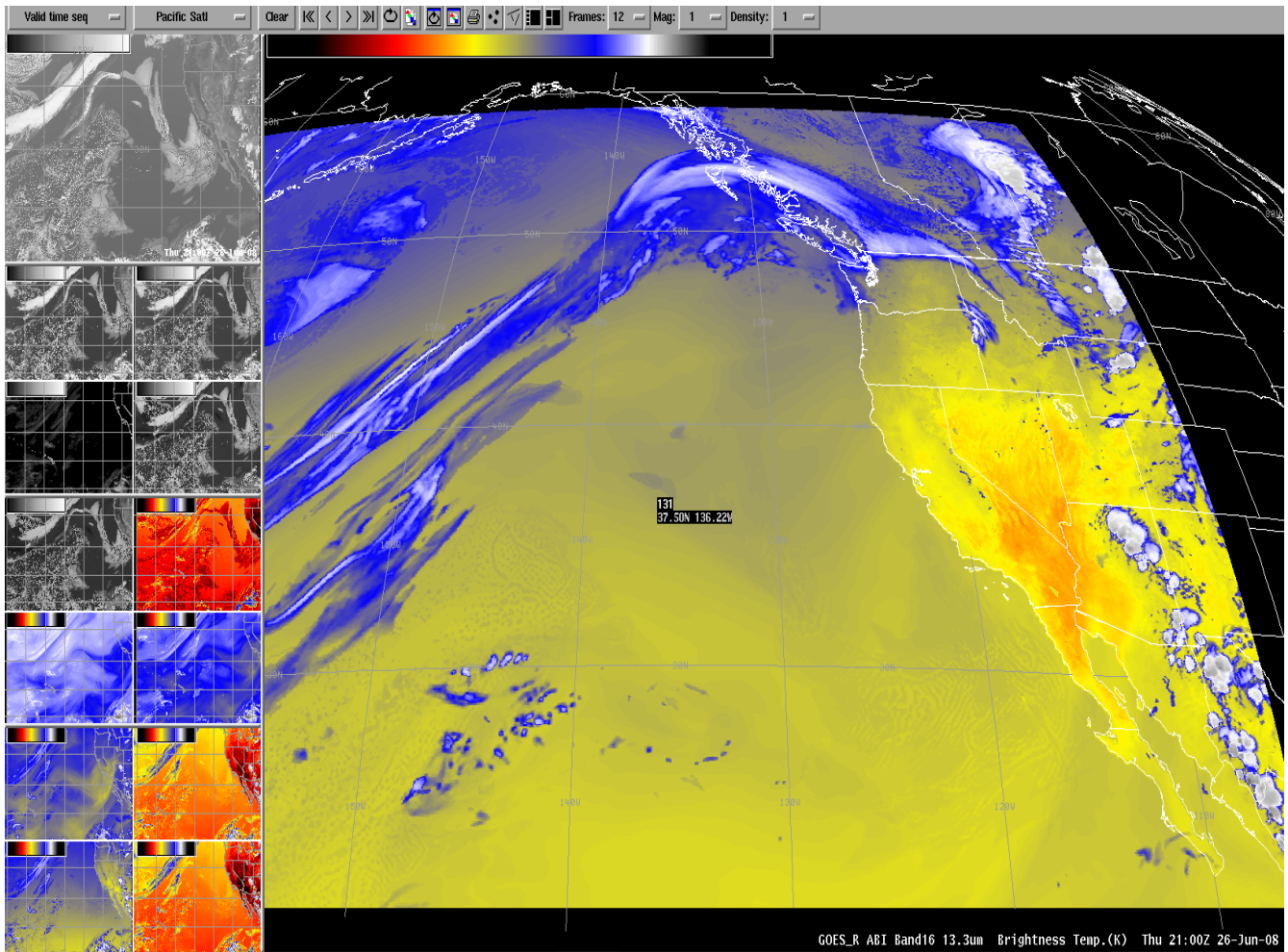
Figure 31. Shows band16 (13.3um) for the pacific projection on 26th-June-2008 at 21:00Z.
