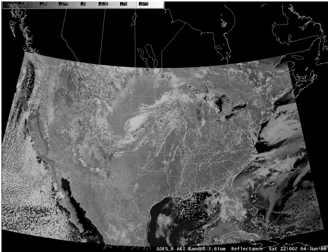
Figure 10. Simulated ABI band 05 (1.6 \mu\text{m} ) for 04 June 2005 at 22:00 UTC.
