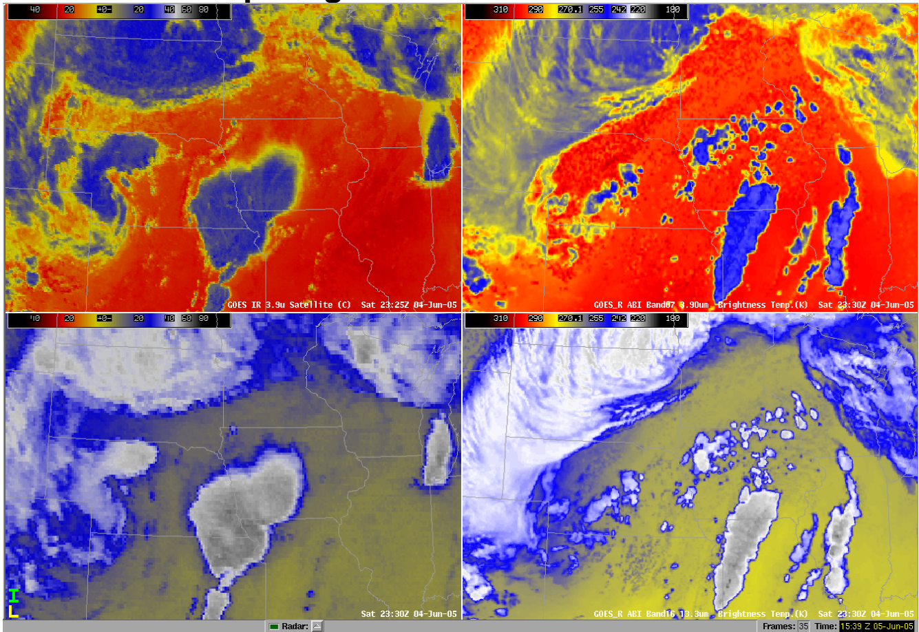
Figure 33. Shows comparison between current GOES and simulated GOES-R ABI bands. The images on the left shows current GOES images from the 3.9um and the 13.3um. The images on the right shows simulated ABI of the corresponding channels. (i.e 3.9 um and 13.3um). Note, of course, that the ABI images are simulated and hence not exactly corresponding to the actual GOES images, although similar features have been resolved.
