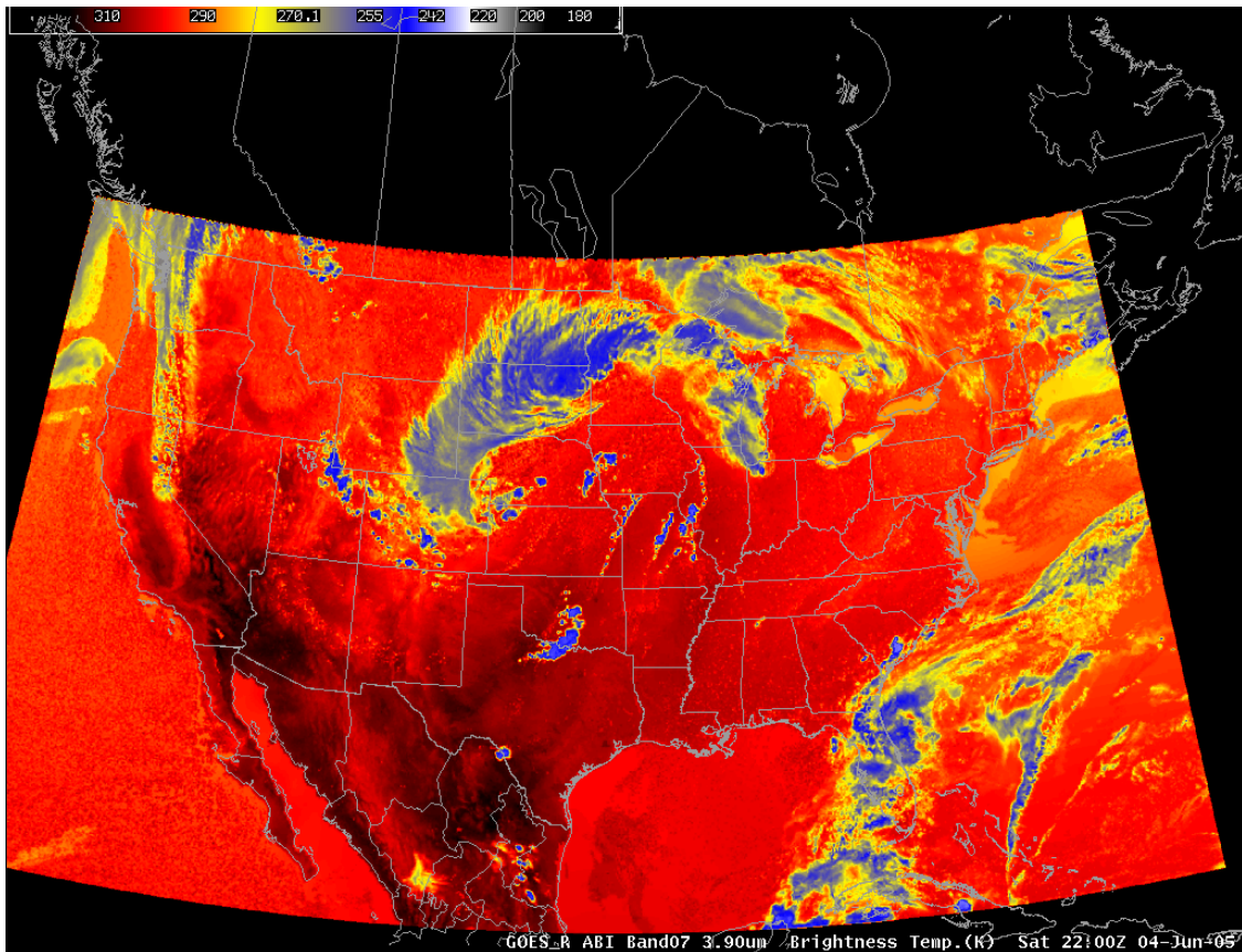
Figure 12. Simulated ABI band 07 (3.9 \mu\text{m} ) for 04 June 2005 at 22:00 UTC.
