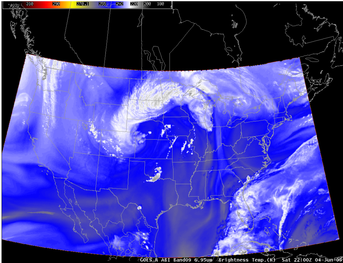
Figure 14. Simulated ABI band 09 (6.95 \mu\text{m} ) for 04 June 2005 at 22:00 UTC.
