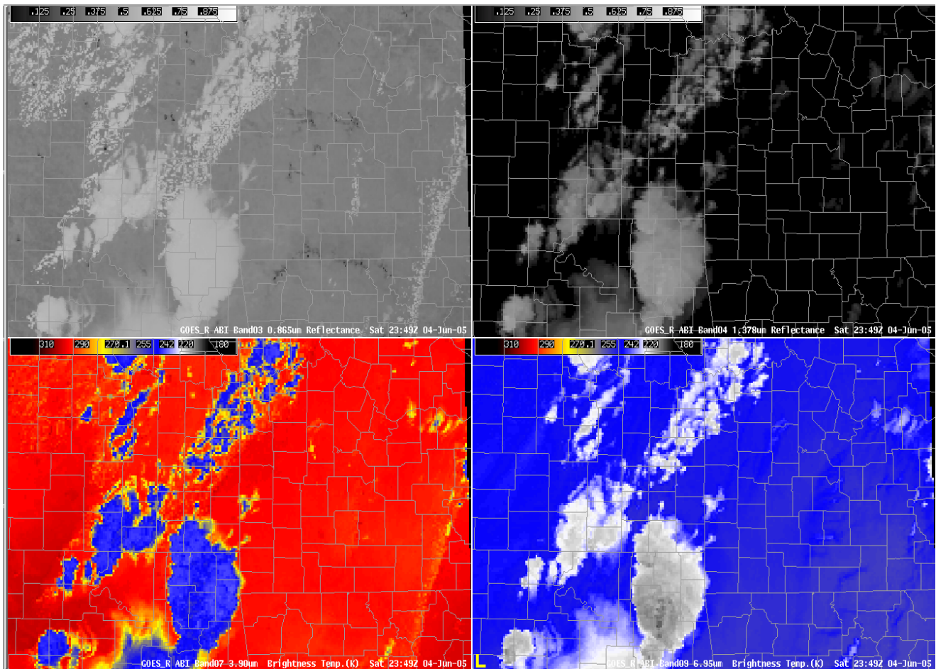
Figure 32. Four of the sixteen ABI bands covering a mesoscale region. The ABI will be able to scan meso scale images every 30 seconds. The bands shown in the image above are: Upper left band03 (0.865um), upper right band04 (1.378um), lower left band07 (3.90um) and lower right band09 (6.95um).
