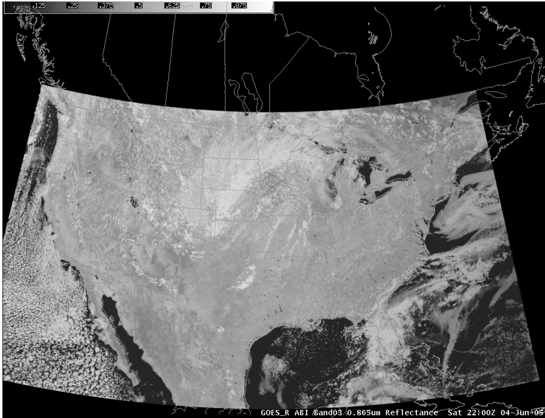
Figure 8. Simulated ABI band 03 (0.865 \mu\text{m} ) for 04 June 2005 at 22:00 UTC.
